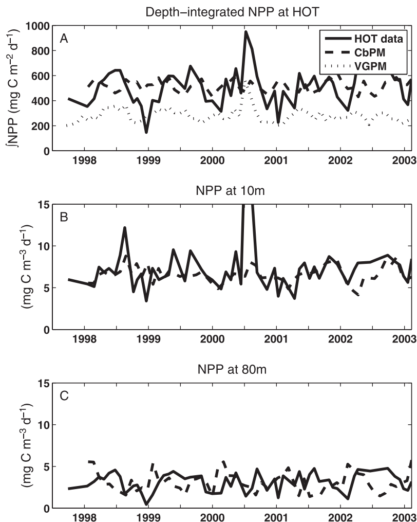
Figure 11. Time series of NPP at HOT site. (a) Water column integrated NPP ( \text{mg C m}^{-2} \text{d}^{-1} ) from ^{14}\text{C} incubations (solid curve), CbPM (dashed curve), and vertically generalized production model (VGPM) (dotted curve). (b) Depth-specific NPP ( \text{mg C m}^{-3} \text{d}^{-1} ) at 10 m. (c) Depth-specific NPP ( \text{mg C m}^{-3} \text{d}^{-1} ) at 80 m.
